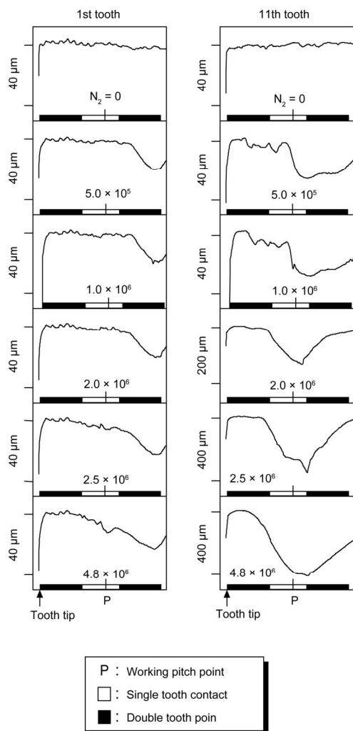
Figure 6. Tooth profile error of pinion during fatigue test: (a) Pinion tooth No. 1; (b) Pinion tooth No. 11.
