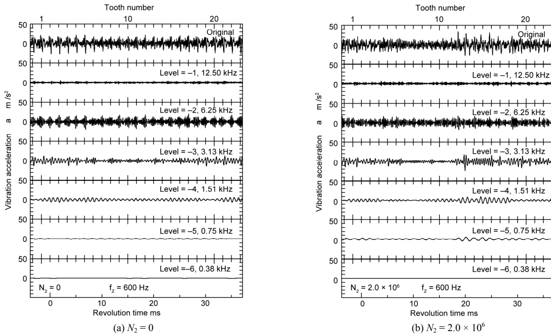
Figure 9. Decomposed vibration acceleration of gear box during fatigue test.
