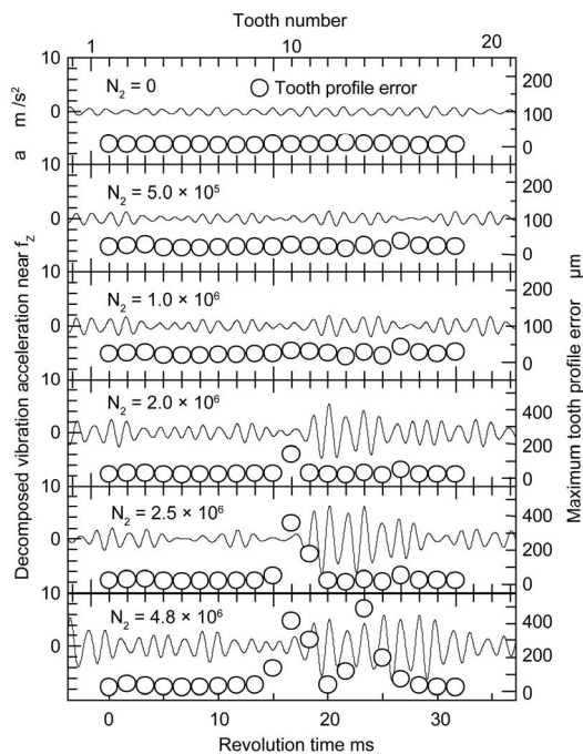
Figure 10. Relation between vibration acceleration and maximum tooth profile during fatigue test.
