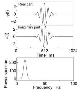
Figure 1. Gabor function.
