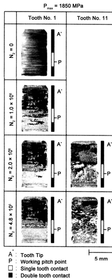
Figure 7. Observation of pinion teeth.
