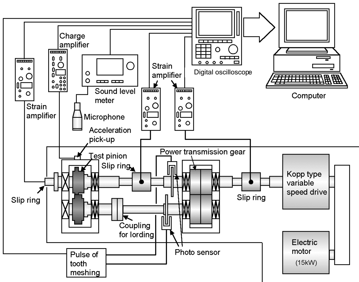
Figure 3. Power circulating gear testing machine.
