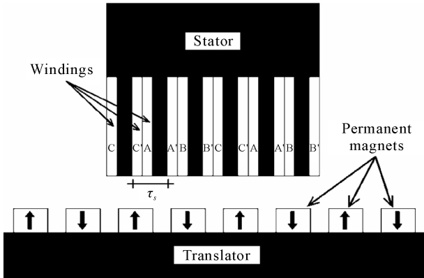
Figure 1. Structure of PMLSM-1.
