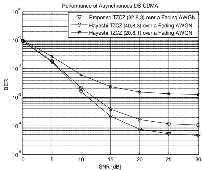
Figure 6. BER performance of Asynchronous DS-CDMA for different TZCZ over a Fading AWGN.
