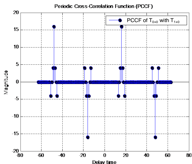
Figure 4. PCCF of T_{0+0} with T_{1+0} .
