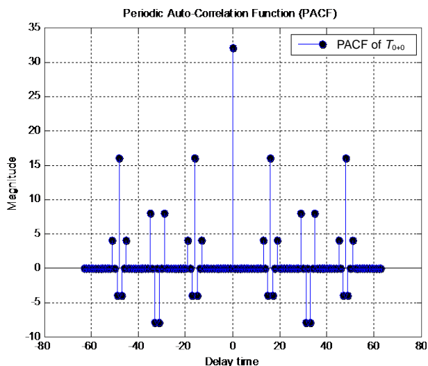
Figure 3. PACF of T_{0+0} .
