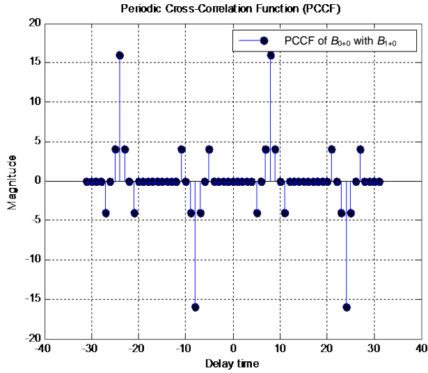
Figure 2. PCCF of B_{0+0} with B_{1+0} .
