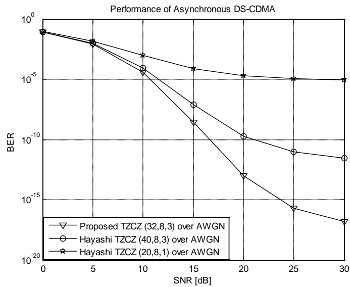
Figure 5. BER performance of Asynchronous DS-CDMA for different TZCZ over AWGN.
