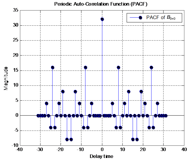
Figure 1. PACF of B_{0+0} .
