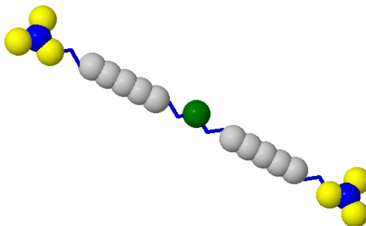
Figure 4. Pharmacophoric groups of compound 1 (CID3526).
