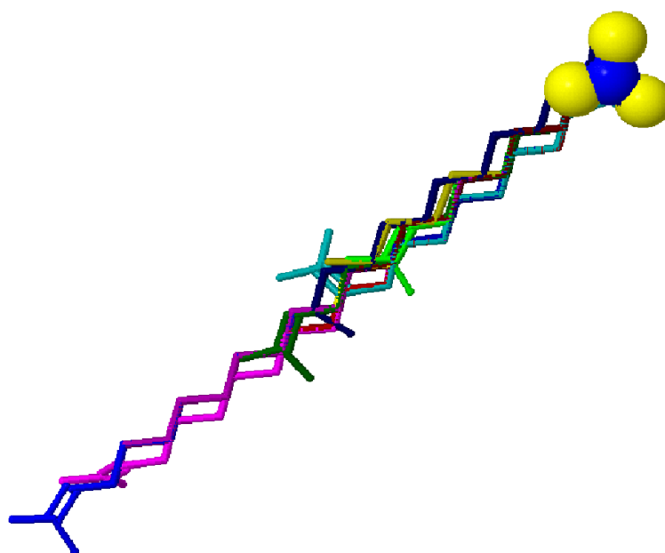
Figure 3. Pharmacophore—alignment of the 15 inhibitors of deoxyhypusine synthase target.
