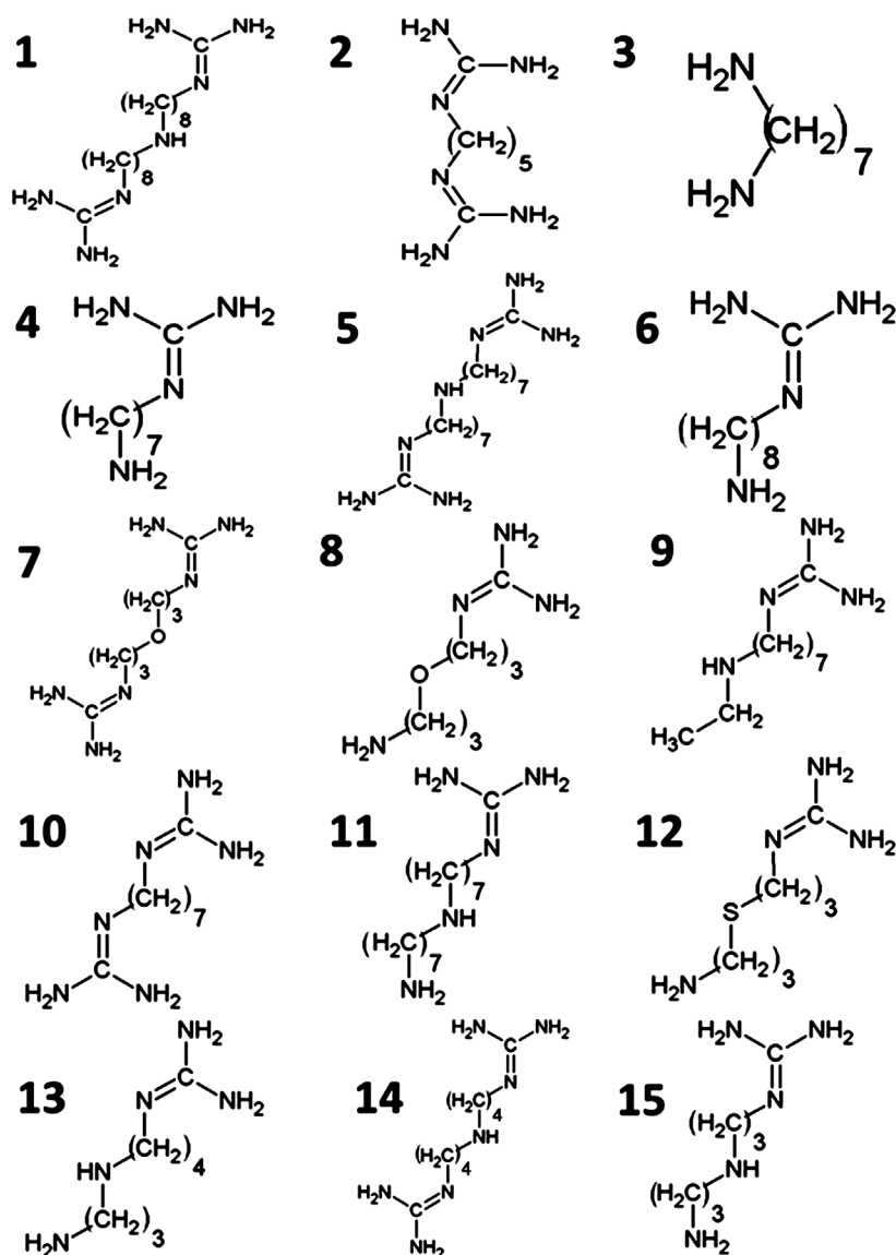
Figure 1. Inhibitors of deoxyhypusine synthase target.
