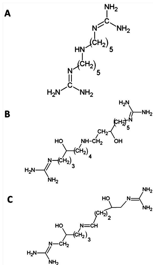
Figure 2. Inhibitors proposed for deoxyhypusine synthase target.
