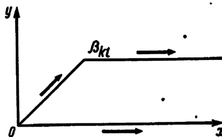
Picture 1. Contour [0, \beta_{k,l}] in complex plane \mathbb{C} .
