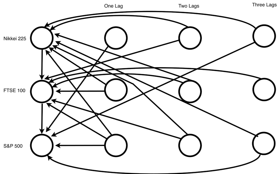
Figure 7. A graphical model fitted to the squared log returns for study period one—28 April 2003 to 29 October 2007.
