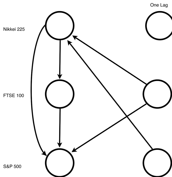
Figure 8. A graphical model fitted to the squared log returns for study period two—30 October 2007 to 11 September 2008.
