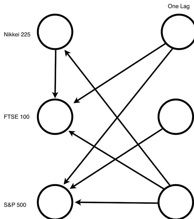
Figure 9. A graphical model fitted to the squared log returns for study period three—1 June 2009 to 2 August 2011.
