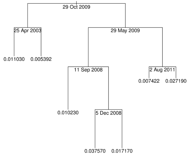
Figure 4. The regression tree for the absolute values of the returns of the S & P 500 stock index.
