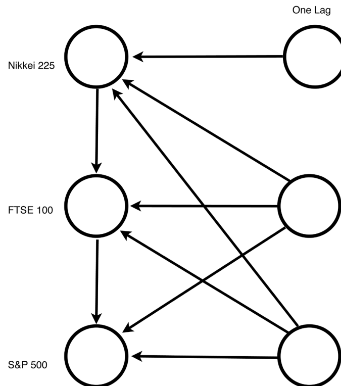
Figure 6. A graphical model of the log returns fitted to the lags. Period one (28 April 2003 to 29 October 2007), two (30 October 2007 to 11 September 2008) and three (1 June 2009 to 2 August 2011) log returns had identical models.
