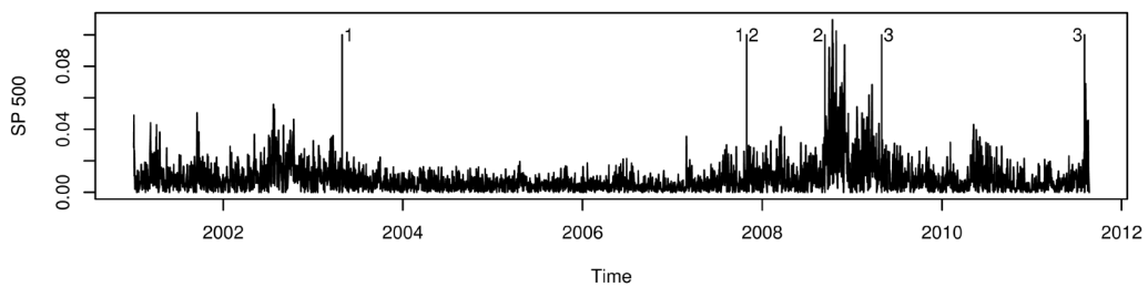
Figure 5. Plots of the absolute values of the log returns of the Nikkei 225, FTSE 100, and S & P 500 stock indices together with the locations of the identified structural breaks.
