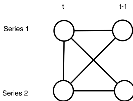
Figure 2. A simple graph with two series and a single time lag.
