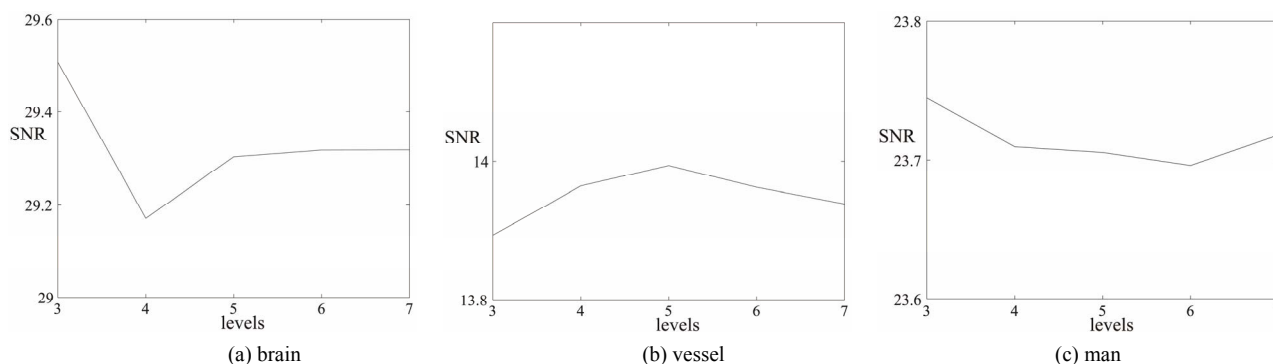
Figure 3. Reconstruction SNR (in dB) of chirp compressed sensing with Daubechies D16 wavelet and different number of levels of wavelet decomposition. The 2D images are not sparsified. The number of measurements taken is 25% of the number of pixels.
