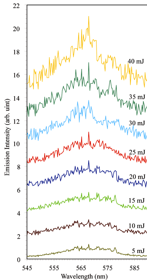
Figure 8. Emission spectra of film sample: 10 -3 mol/l R6G:10 -3 mol/l at different pumping energies.
