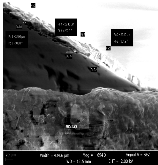
Figure 2. Image of SEM for measuring thickness sample as film.
