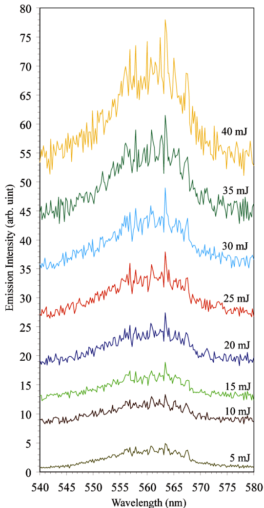
Figure 6. Emission spectra of liquid sample: 10 -5 mol/l R6G:10 -3 mol/l at different pumping energies.
