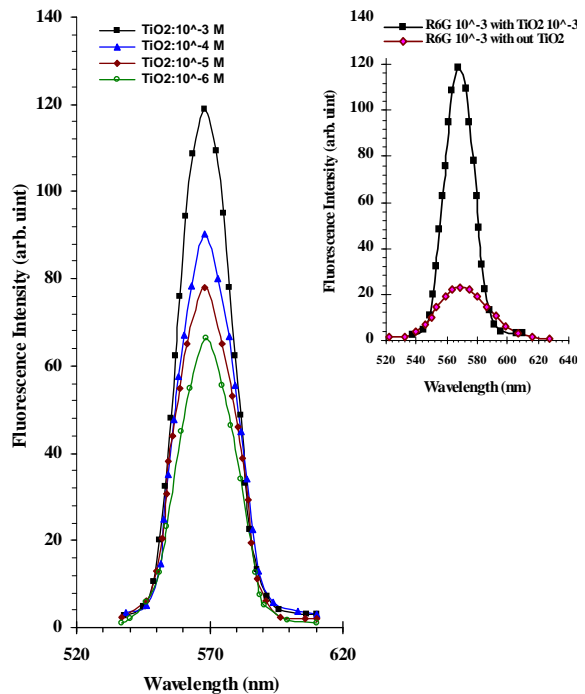
Figure 5. The fluorescence spectra of film samples with 10^{-3} mol/l R6G and 10^{-3} , 10^{-4} , 10^{-5} , 10^{-6} mol/l hosted by polymer PMMA.
