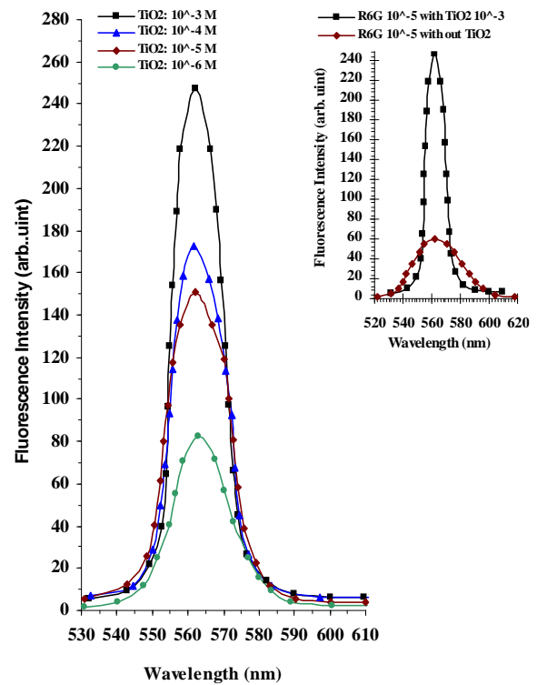
Figure 4. The fluorescence spectra of liquid sample with 10^{-5} mol/l R6G and 10^{-3} , 10^{-4} , 10^{-5} , 10^{-6} mol/l hosted by polymer PMMA.
