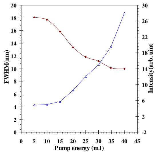
Figure 7. Random laser threshold determined from the relation of maximum intensity and FWHM at different of pumping energies for a liquid sample : 10 -5 mol/l R6G: TiO 2 10 -3 mol/l.
