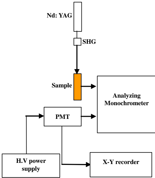
Figure 3. Schematic diagram of RL experimental setup.
