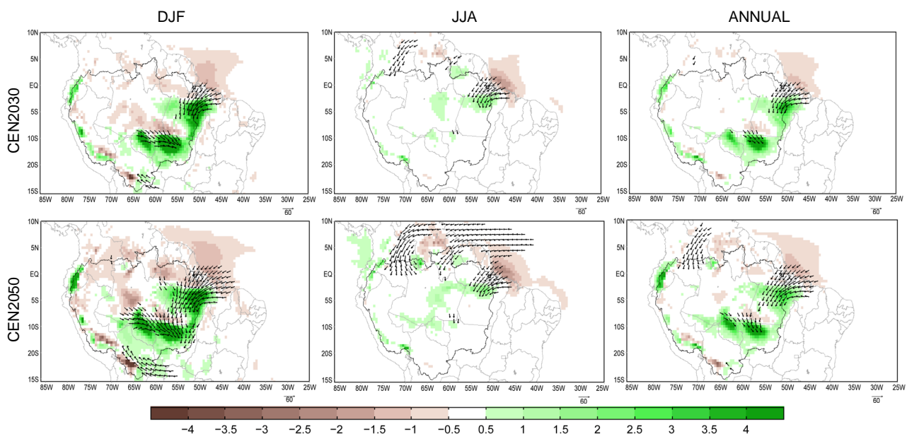
Figure 2. Precipitation (shaded, units: mm/day) overlaid with vertically integrated moisture flux (vectors, units: \text{g/kg}\cdot\text{m/s}\cdot\text{hPa} ) for summer (DJF), winter (JJA) and Annual based on difference between deforestation and control runs. Magnitude above 20 \text{g/kg}\cdot\text{m/s}\cdot\text{hPa} vector is displayed.
