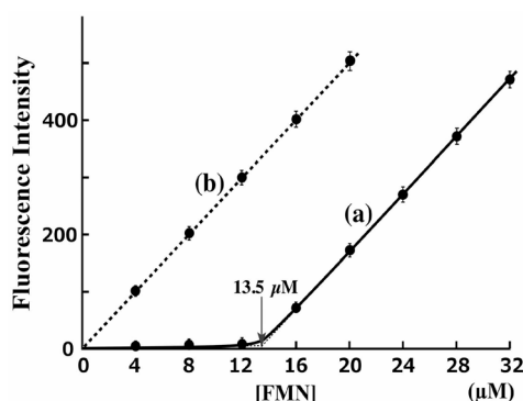
Figure 3. Fluorescence emission response at various concentrations of FMN in the presence of 13.5 μM Dabcyl-labeled Phos-tag ligand and 0.10 mM ZnCl 2 : (a) With no additive and (b) in the presence of 2.0 mM EDTA. Fluorescence intensities at 530 nm with excitation at 350 nm at 25°C and pH 7.4 (10 mM Hepes-NaOH, 0.10 M NaCl).
