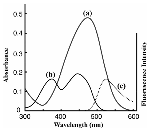
Figure 2. Absorption spectra at 25°C and pH 7.4 (10 mM Hepes-NaOH, 0.10 M NaCl): (a) Mixture of 15 μM Dabcyl-labeled Phos-tag ligand and 50 μM ZnCl 2 , \lambda_{\text{max}} = 475 \text{ nm} ( \epsilon = 32,000 \text{ M}^{-1}\cdot\text{cm}^{-1} ); (b) 15 μM FMN, \lambda_{\text{peak1}} = 373 \text{ nm} ( \epsilon = 10,500 \text{ M}^{-1}\cdot\text{cm}^{-1} ), \lambda_{\text{peak2}} = 445 \text{ nm} ( \epsilon = 12,500 \text{ M}^{-1}\cdot\text{cm}^{-1} ); (c) Fluorescence spectrum of 15 μM FMN with excitation at 350 nm at 25°C and pH 7.4 (10 mM Hepes-NaOH, 0.10 M NaCl): \lambda_{\text{em}} = 525 \text{ nm} .
