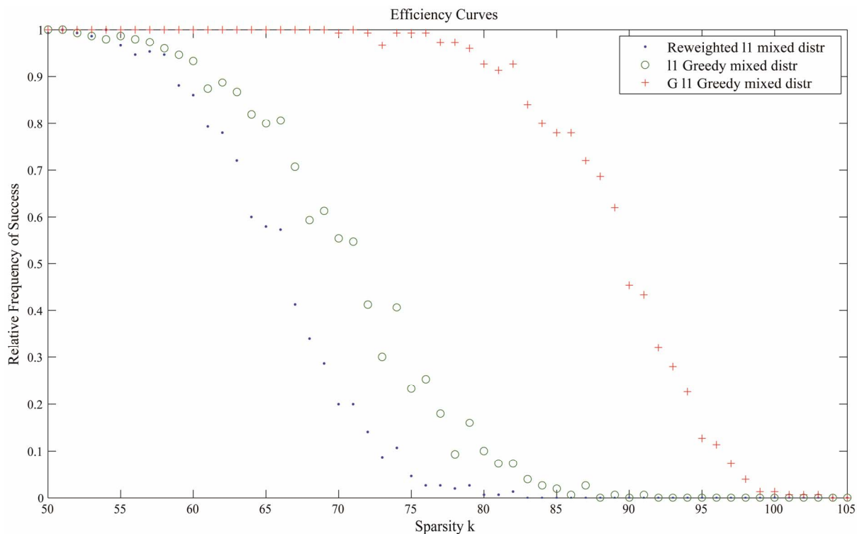
Figure 6. Improvements in recovering sparse solutions with a mixed Gaussian distribution from the generalized l_1 greedy algorithm when compared to the reweighted l_1 -minimization and l_1 greedy algorithms.
