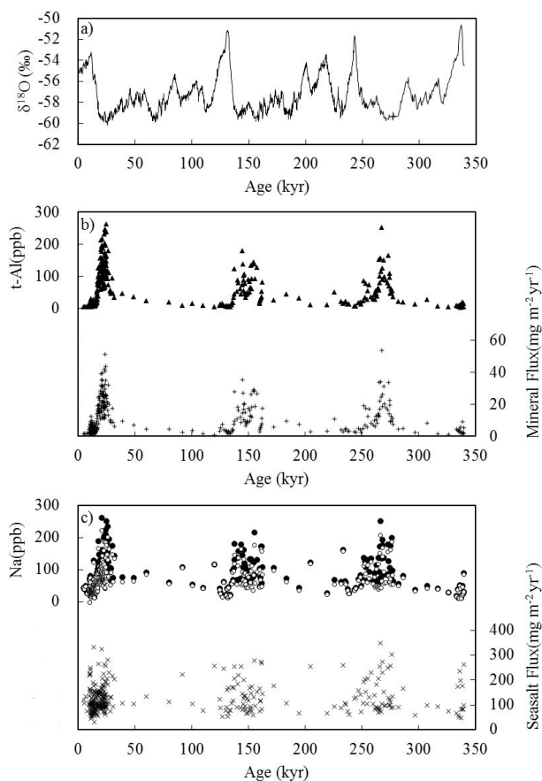
Figure 1. Profiles of (a) \delta^{18}\text{O} (Kawamura et al. , 2007); (b) t-Al concentration (closed triangles) and mineral flux (plus signs); and (c) t-Na concentration (closed circles), sea-salt-Na concentration (open circles) and sea-salt flux (crosses) of the Dome Fuji ice core during the past 340 kyr.
