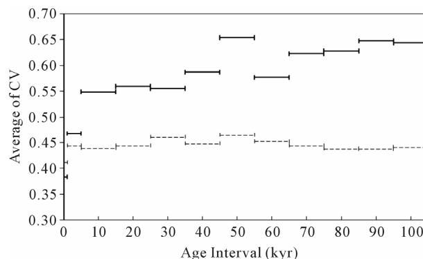
Figure 2. Average of coefficients of variation (CV) of mineral (solid lines) and sea-salt (dashed lines) fluxes to Dome Fuji in various age intervals.
