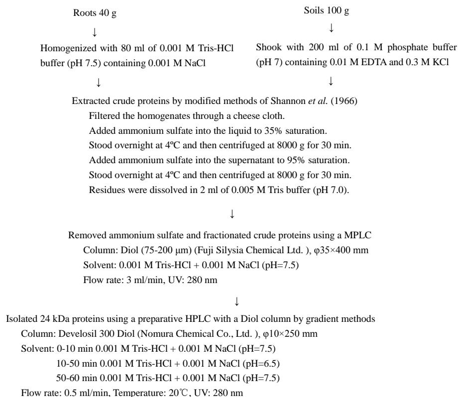
Figure 1. Procedures for the extraction and purification of proteins in roots and soils.
