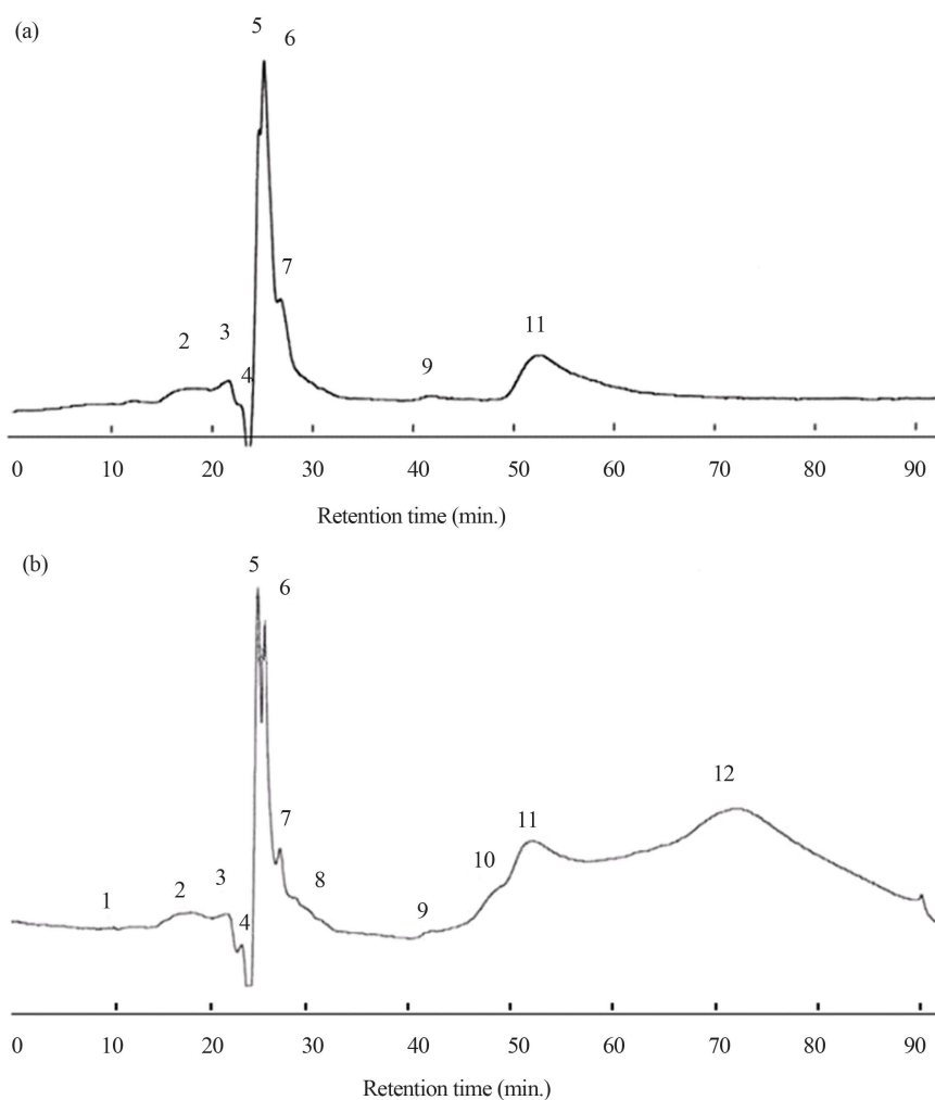
Figure 5. Chromatogram of soil proteins fractionated by HPLC. (a) Isochromatic methods Column: Develosil 300 Diol, \phi 10 × 250 mm, Solvent: 0.001 M Tris-HCl + 0.001 M NaCl (pH = 7.5), Flow rate: 0.5 ml/min, Temperature: 20°C, UV: 280 nm; (b) Gradient methods (see in Figure 1).
