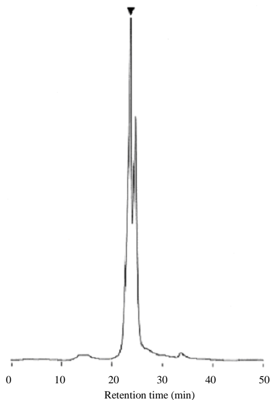
Figure 6. A chromatogram of 24 kDa proteins of Glomus intraradices -inoculated soybean roots fractionated by gradient HPLC. Gradient methods: see in Figure 1 . The black arrow shows 24 kDa proteins in the electrophoresis with SDS plates.
