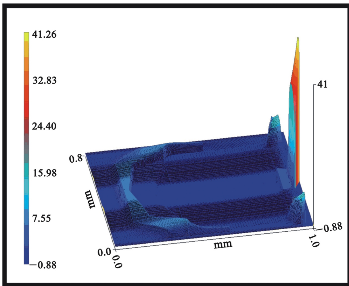
Initial Air Bearing Slider Normalized Pressure Profile
