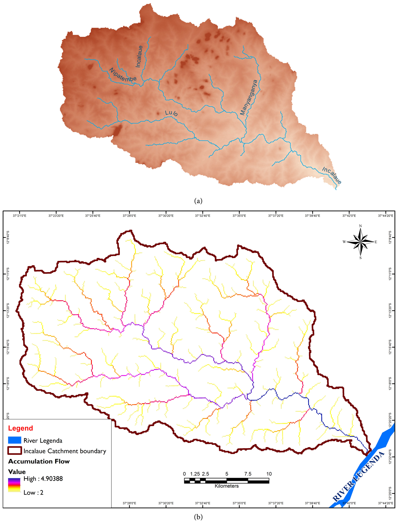
Figure 3. Hill-slope map (a) and flow accumulation map (b).
