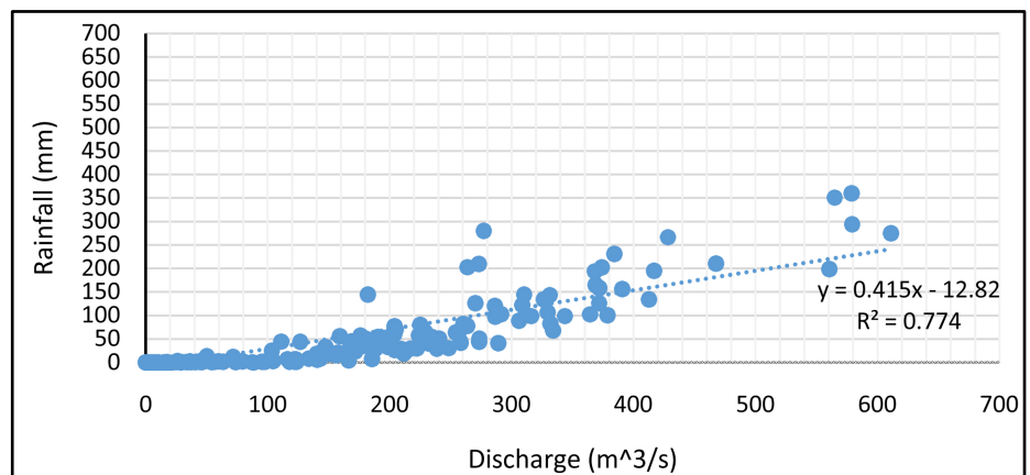
Figure 9. Rainfal-runoff model using NASA-POWER data.
