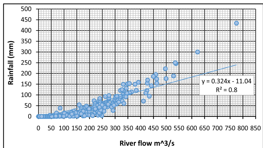
Figure 5. Rainfall-runoff relationship generated using FAO dataset for the period (1980–2014).
