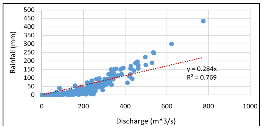
Figure 11. Rainfall-runoff model using gauged data.
