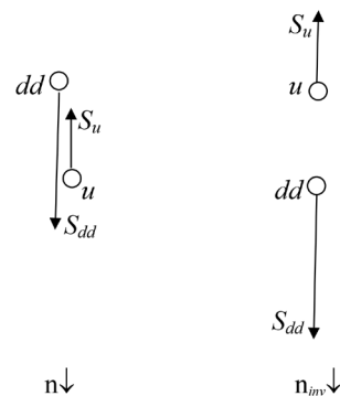
Figure 4. Schematic configuration of the spin \downarrow\downarrow component of a triplet dineutron {}^2n_1 . The right neutron configuration is the same as that in Figure 2 . The left neutron configuration is the same as that in Figure 3 .
