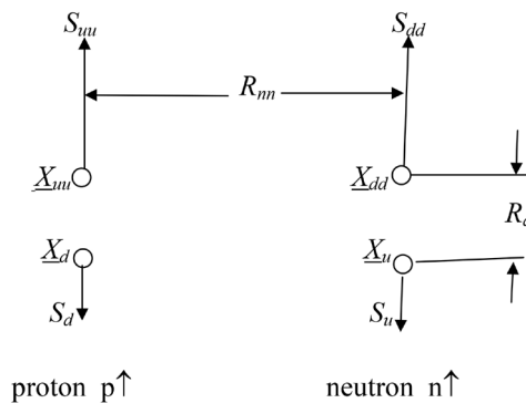
Figure 1. Schematic configuration of the spin \uparrow\uparrow component of a triplet deuteron {}^2H_1 . \underline{x} denotes the coordinate and S the spin of the diquarks and quarks. The subscripts refer to the quark content. S_{uu} = S_{dd} = 1 and S_u = S_d = -1/2 with signs given by the arrow \uparrow for + and \downarrow for - . \underline{x}_{uu} = \underline{x}_u and \underline{x}_d = \underline{x}_d in [3] (10.1.1) or [4] (A2). R_a \approx 3.23 fm [5] (2.5) is the mean value of the diquark-quark distance. The neutron configuration is obtained from the proton configuration via the interchange u \leftrightarrow d . R_{nn} is distance between the both nucleons.
