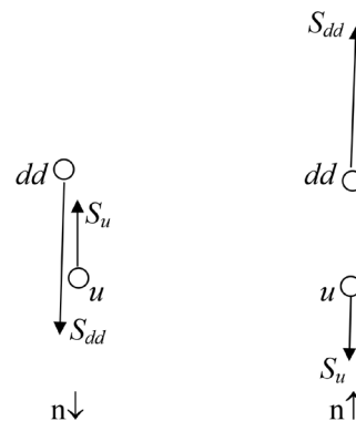
Figure 3. Schematic configuration of a singlet dineutron {}^2n_0 . The right neutron configuration is the same as that in Figure 1 . Switching the spin directions in n \uparrow on the right leads to the n \downarrow configuration on the left.
