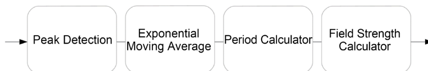
Figure 4. Digital signal processing flow diagram.
