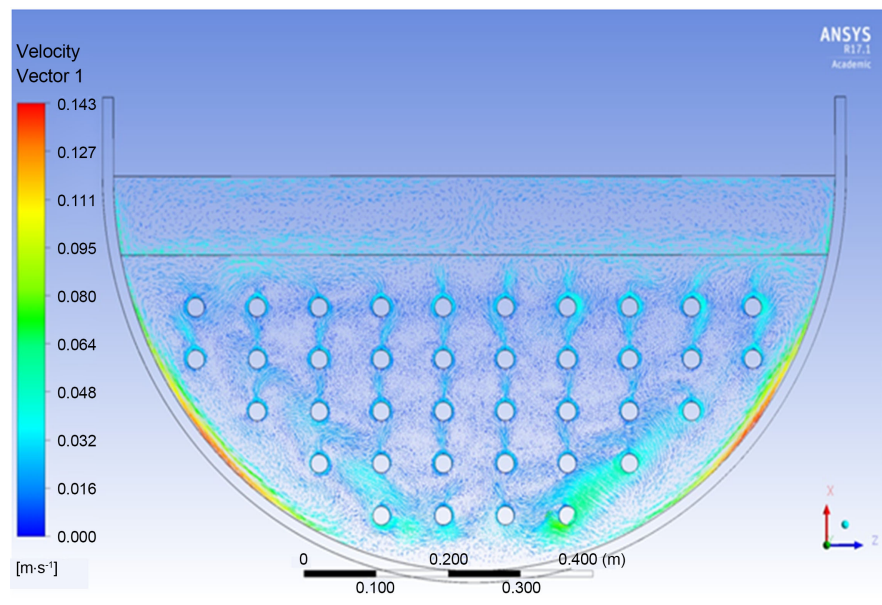
Figure 6. Velocity field in the molten pool.
