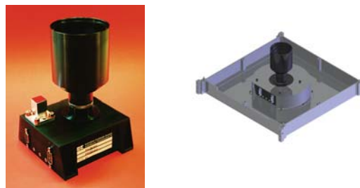
Fig 8 Star Sensor KM 1301 and its integration into the tray structure
