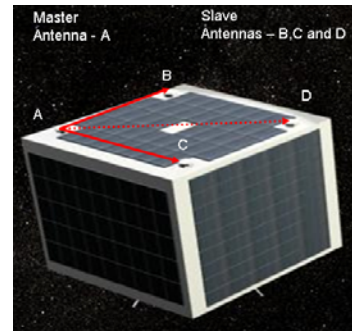
Fig 7 SPARx antenna array for JAESat 3-axis attitude determination. antenna D will be optional
