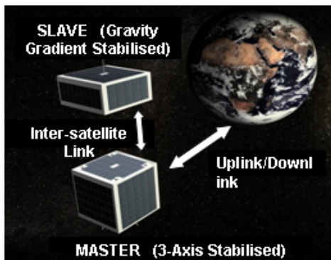
Fig 4 JAESat Communication Concept
