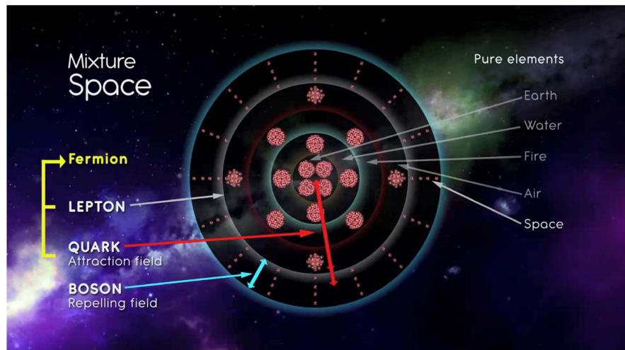
Figure 12. Pure element arrangement in Mixture Space.
