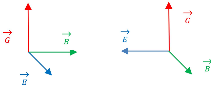
Figure 28. Interaction forces of two I-particles in attraction.
