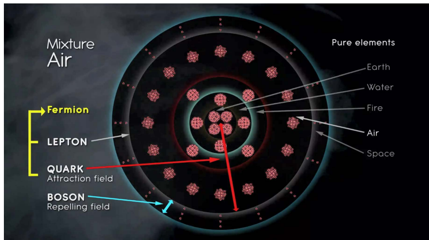
Figure 13. Pure element arrangement in Mixture Air.
