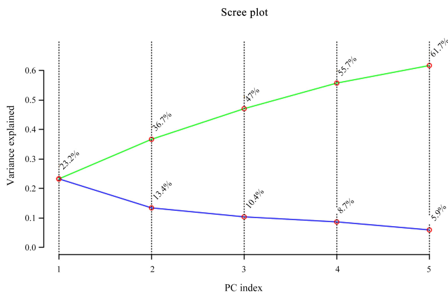
Figure SM1. The variations that explained by PCs from PCA modeling of VOC profiles from American, Chinese and two backcross hybrids generations of chestnut.
