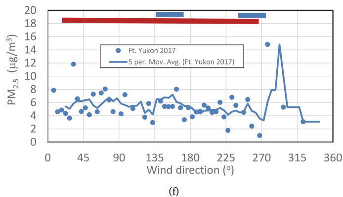
Figure 12. 5°-sector mean concentrations of (a) sulfate, (b) ammonium vs. wind direction as observed in 2008/09 at three sites in the FMA in the 2008/09 cold season. September to April 5°-sector mean [PM_{2.5}] vs. wind direction at the villages of (c) Beaver, (d) Chalkyitsik, (e) Circle and (f) Ft. Yukon. See Figure 1 for locations. Wind direction sectors marked with red and blue bars indicate wind direction sectors for which the sites are in the downwind of the village and hot springs, respectively.
