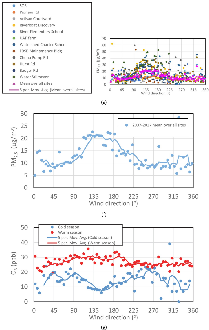
Figure 9. 2005-2014 mean speciation of PM 2.5 and PM 2.5 relationships to meteorology of (a) selected species vs. temperature, (b) 2007-2018 PM 2.5 from all sites vs. mean wind speed in 0.01, 0.1 and 0.5 m·s -1 bins and respective polynomial fits (lines) of y = -0.608x^5 + 7.3687x^4 - 32.671x^3 + 64.099x^2 - 54.139x + 22.49 , y = -0.7683x^5 + 9.3061x^4 - 41.213x^3 + 80.951x^2 - 68.613x + 26.253 , y = -0.2393x^6 + 2.0569x^5 - 2.6148x^4 - 21.151x^3 + 74.983x^2 - 82.772x + 32.427 with R 2 of 0.512, 0.808, 0.940, (c) 2011-2014 SO 2 , sulfate vs wind direction in 5° sector bins, (d) 2005-2014 climatology of nitrate, sulfate, and non-metals (NM) vs. wind direction in 5°-sector bins, (e) 2007-2017 PM 2.5 at all sites in the FMA and mean over all sites as function of wind direction in 5°-sector bins, (f) 2007-2017 mean PM 2.5 averaged over all sites in the FMA as a function of wind direction. (g) Warm and cold season O 3 vs. wind direction. Lines are 5-values running means.
