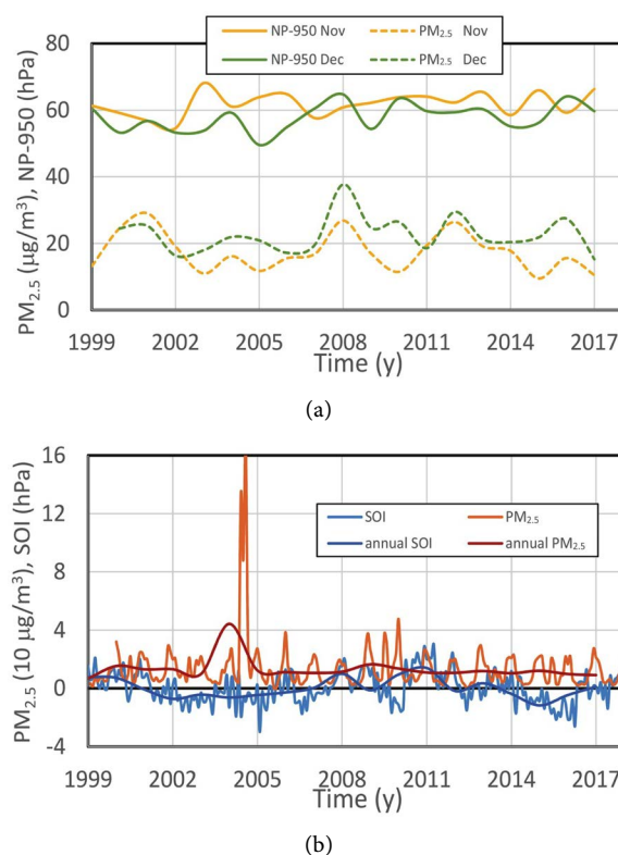
Figure 7. November and December 1999–2017 climatology of (a) monthly means of NP-950 hPa and [PM_{2.5}] , and (b) monthly and annual means of SOI and 0.1 [PM_{2.5}] .
