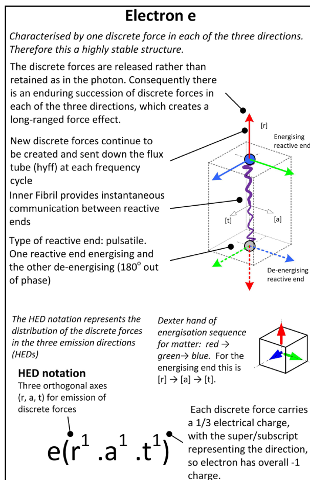
Figure 2. The representation of the electron's internal and external structures. It is proposed that the particle has three orthogonal discrete forces, energised in turn at each reactive end. Adapted from [20].
