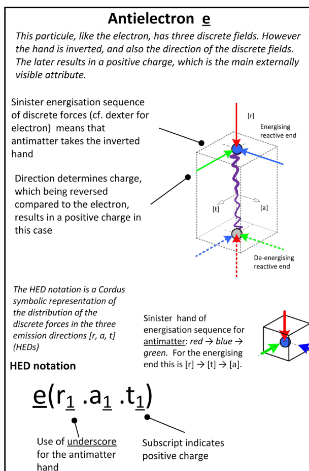
Figure 3. The representation of the antielectron as per the Cordus theory. The antimatter attribute, which is opposite to that of the electron, arises from the handedness of energisation sequence of the three orthogonal discrete forces. The charge is also opposite to that of the electron, and this arises as the direction of the discrete forces is also reversed. Adapted from [21].
