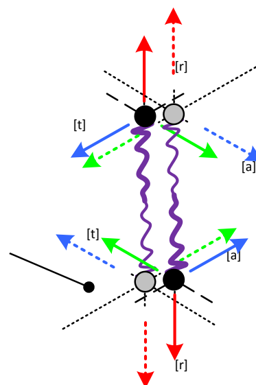
Figure 6. Proposed structure of the Pauli pair, whereby two electrons are bonded with a transphasic interaction.
