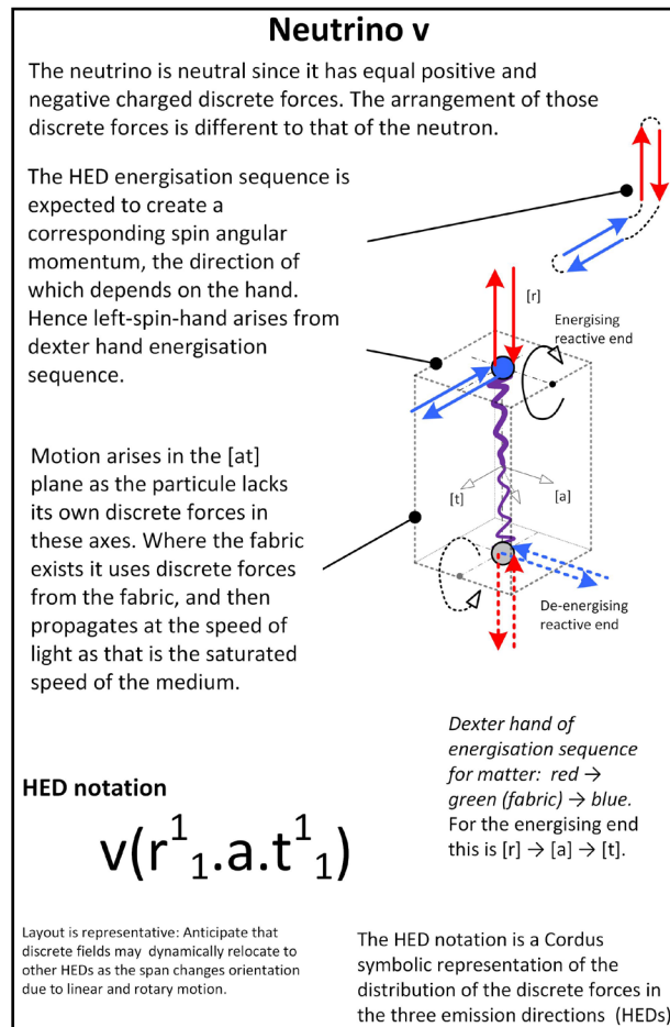
Figure 4. Predicted structure of the neutrino. This physical structure also conceptually explains why this particle must have motion, and why its direction of spin is coupled to the matter-antimatter attribute. Adapted from [22].
