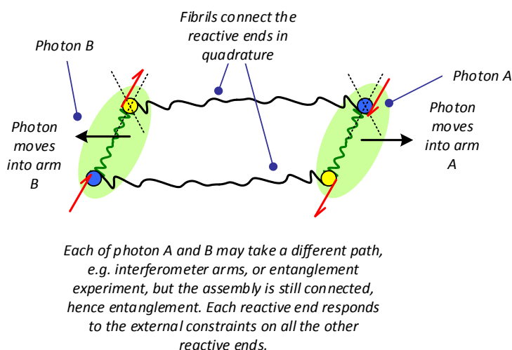
Figure 5. Qualitative explanation of two-photon entanglement. The photons are predicted to originate from a Pauli pair of electrons—these electrons are bonded in a transphasic interaction and hence their emitted photons also have that interaction. Consequently the four reactive ends of the two photons are linked by fibrils, even as they move further apart. As a result the behaviours of the photons are coupled: hence entanglement.
