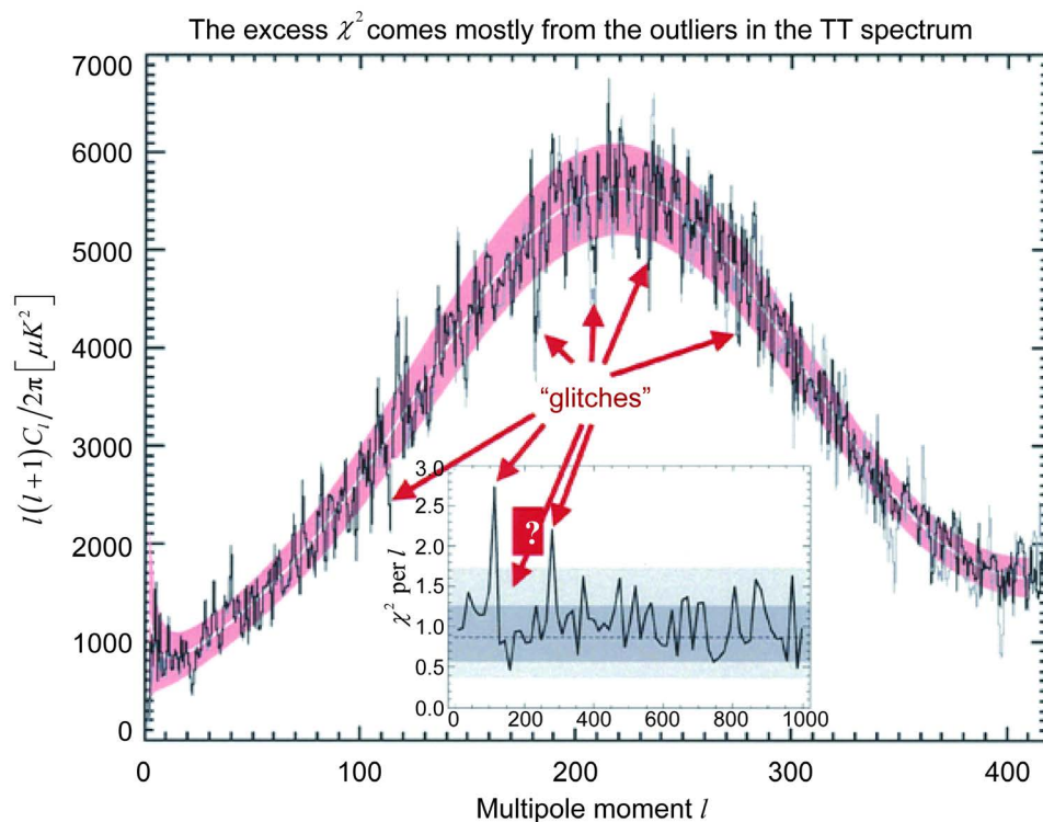
Figure A1. Is the primordial density perturbation really scale-free?
