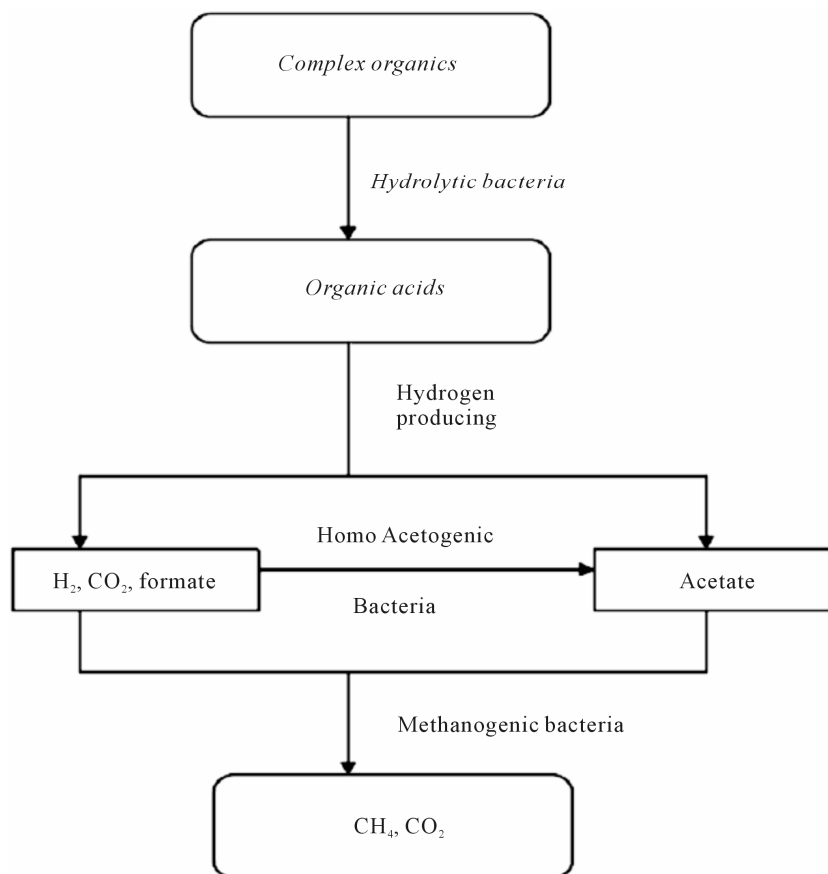
Figure 3. Biogas production process [15].
