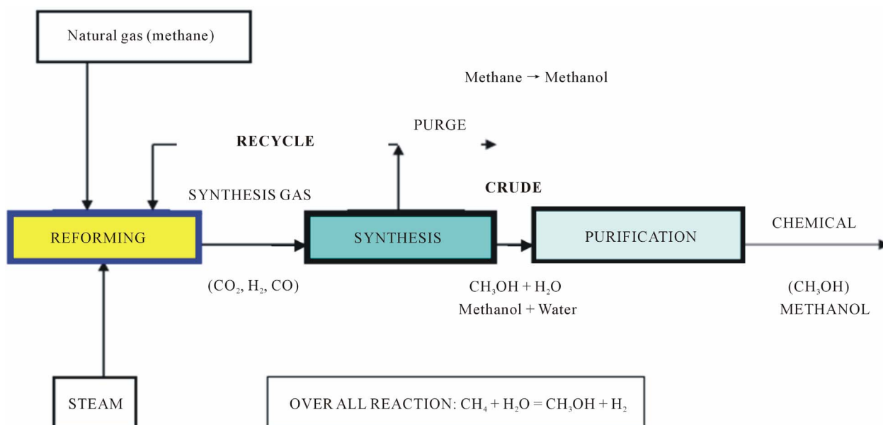
Figure 2. Schematic diagram shows methanol production [8].
