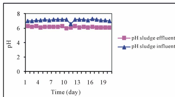
Figure 6. pH sludge before and after treatment in the digester [18].
