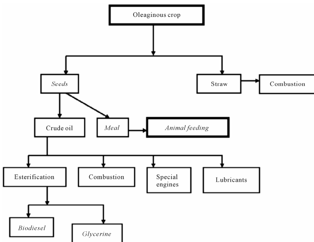
Figure 9. Flow chart of biodiesel production [20].
