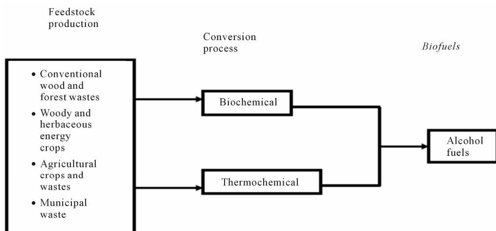
Figure 8. Biofuel pathways for renewable alcohol fuels [19].
