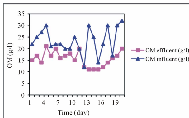
Figure 5. Organic matters before and after treatment in digester [18].
