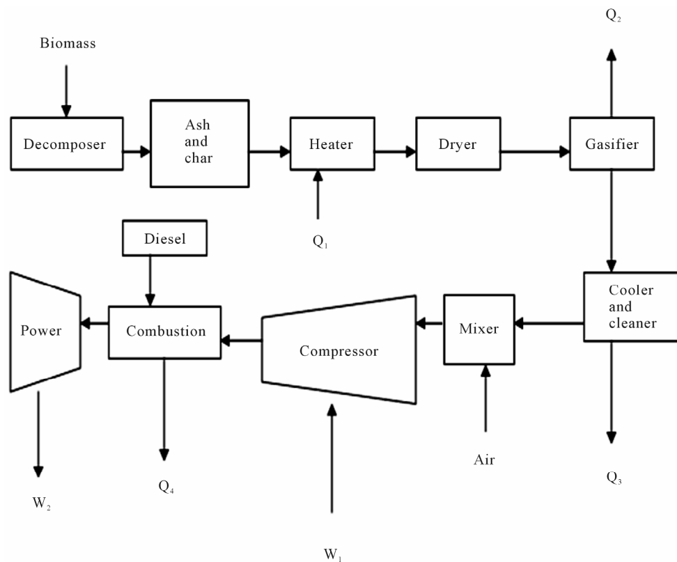
Figure 7. Advanced biomass power with diesel engine [19].
