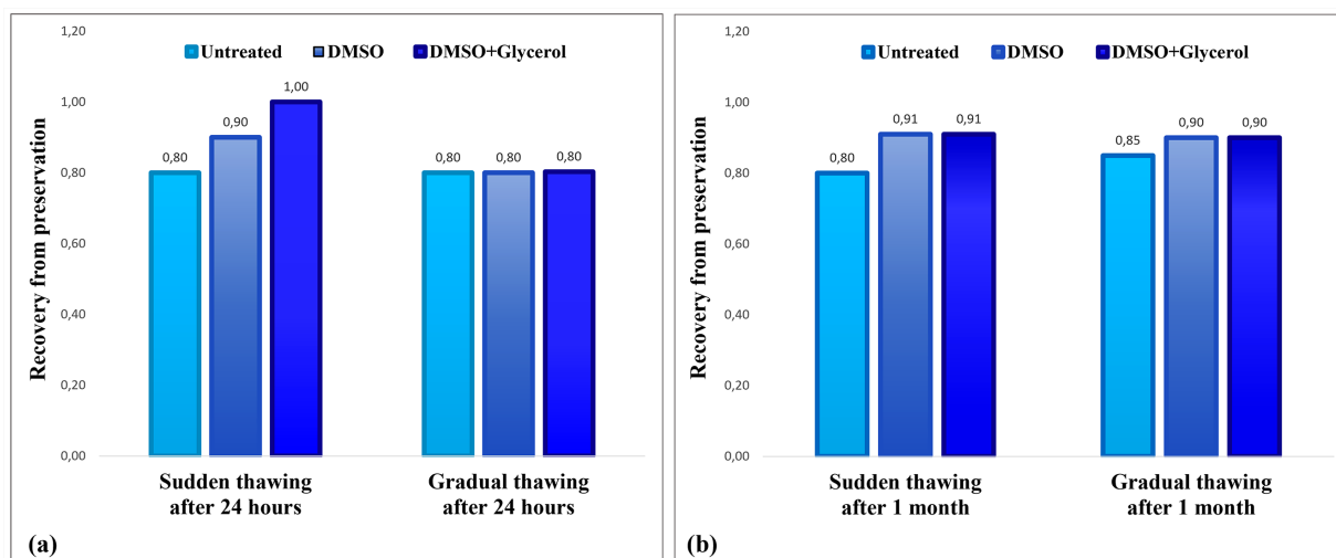
Figure 2. Results of growth recovery from different preservation strategies of Sticococcus bacillaris . (a) recovery after 24 hours of storage, (b) recovery after 1 month of storage. Untreated: cryopreserved untreated control sample; DMSO: sample cryopreserved using dimethyl sulfoxide; DMSO + Glycerol: sample cryopreserved using dimethyl sulfoxide and glycerol.
