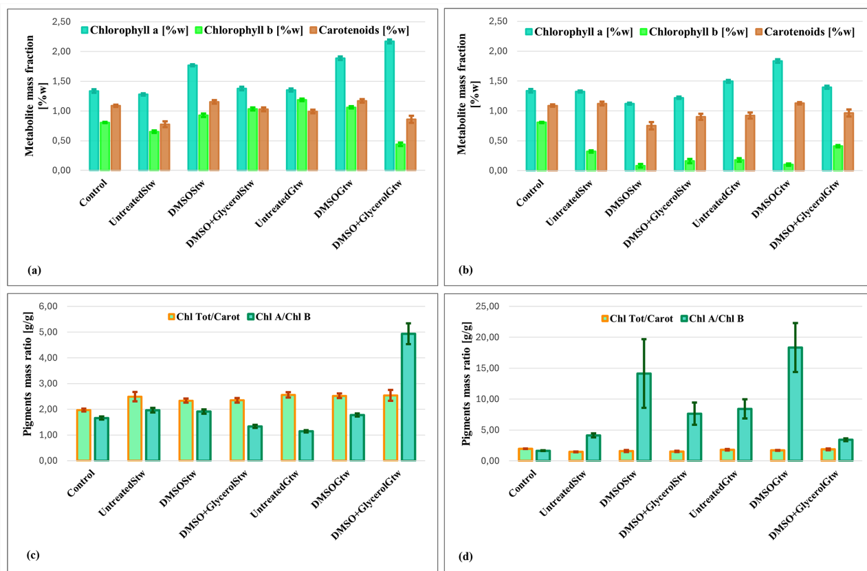
Figure 4. Results of the pigments mass fraction of the biomass: pigments mass fraction [%w] of the biomass after 24 hours of storage (a), and after 1 month of storage (b), total chlorophylls to carotenoids ratio (Chl Tot/Carot) and chlorophyll a to chlorophyll b ratio (Chl A/Chl B) after 24 hours of storage (c), and after 1 month of storage (d).
