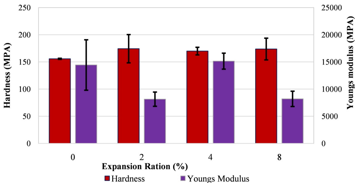
Plot of Hardness and Youngs modulus Vs. Expansion Ratio
