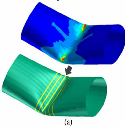
Laser track design based on maximum plastic deformations
