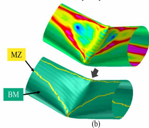
Laser track design based on maximum principal stress
