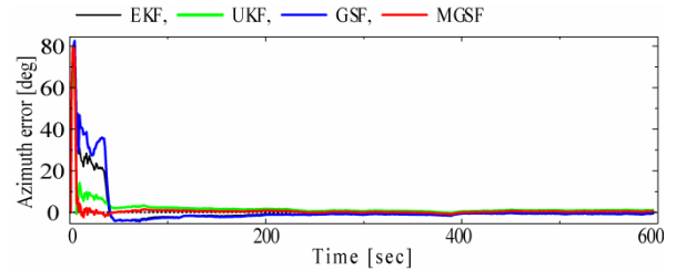
Fig. 7. Azimuth errors
