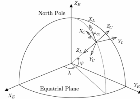
Fig. 2. Coordinate frames
