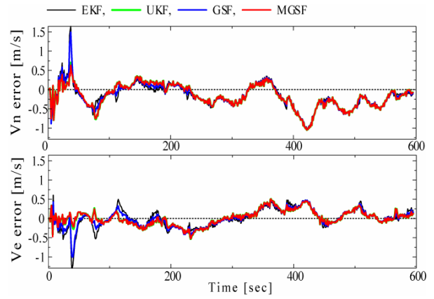
Fig. 6. Velocity errors
