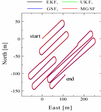
Fig. 4. Positioning results
