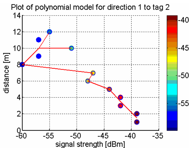
Fig. 3. Relationship between the measured signal strength and the distance along a baseline described by a polynomial model of order p = 8
