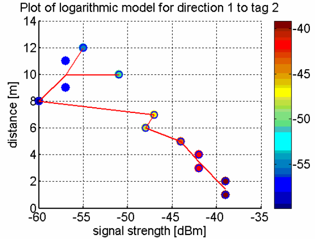
Fig. 1. Relationship between the measured signal strength and the distance along a baseline described by a logarithmic model of order p = 8
