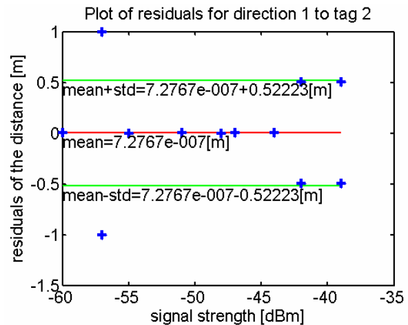
Fig. 4. Residuals between the polynomial model and the measured signal strength along a baseline
