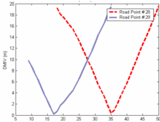
Fig. 6. The minimum of the difference between the measured GPS pseudorange and the geometrical range to one satellite arises when the GPS receiver is nearest to the road point's location (after Mok et al., 2007)
