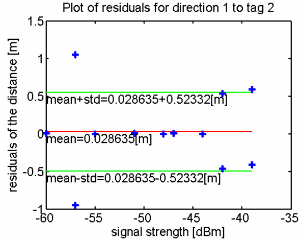
Fig. 2. Residuals between the logarithmic model and the measured signal strength along a baseline
