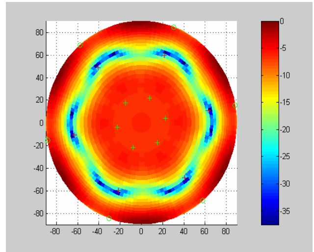
Figure 8. Beam pattern overview for GPS signals (15, 10), (15, 70), (15, 130), (15, 190), (15, 250), (15, 310). Pseudolite signals (85, 10), (85, 70), (85, 130), (85, 190), (85, 250), (85, 310) and interference (45, 10), (45, 70), (45, 130), (45, 190), (45, 250), (45, 310).
