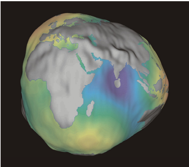
Fig. 2 Global gravity field model from three months of CHAMP data only
