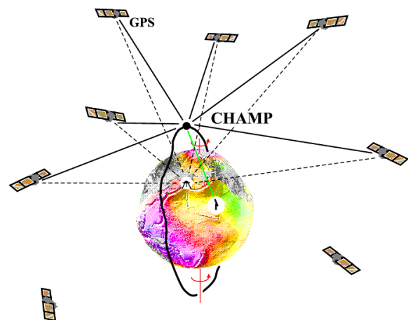
Fig. 1 High-low GPS-CHAMP satellite-to-satellite tracking for gravity field recovery
