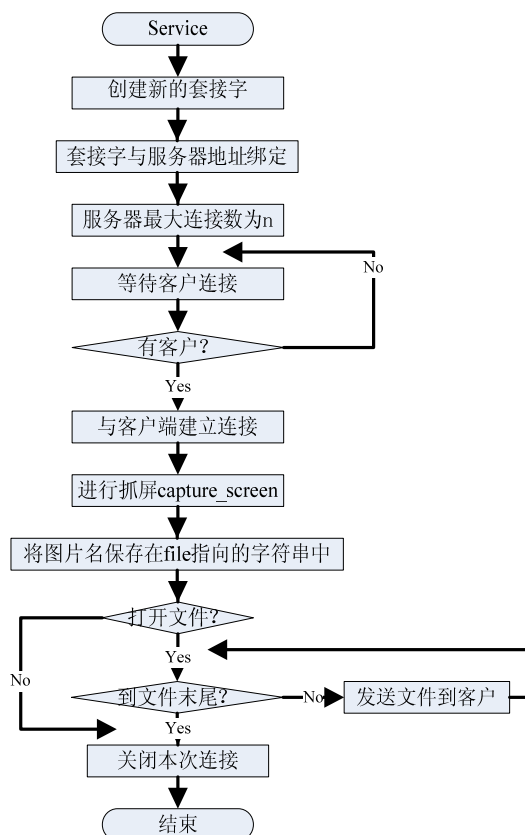
Figure 2. Flowchart: Server process
